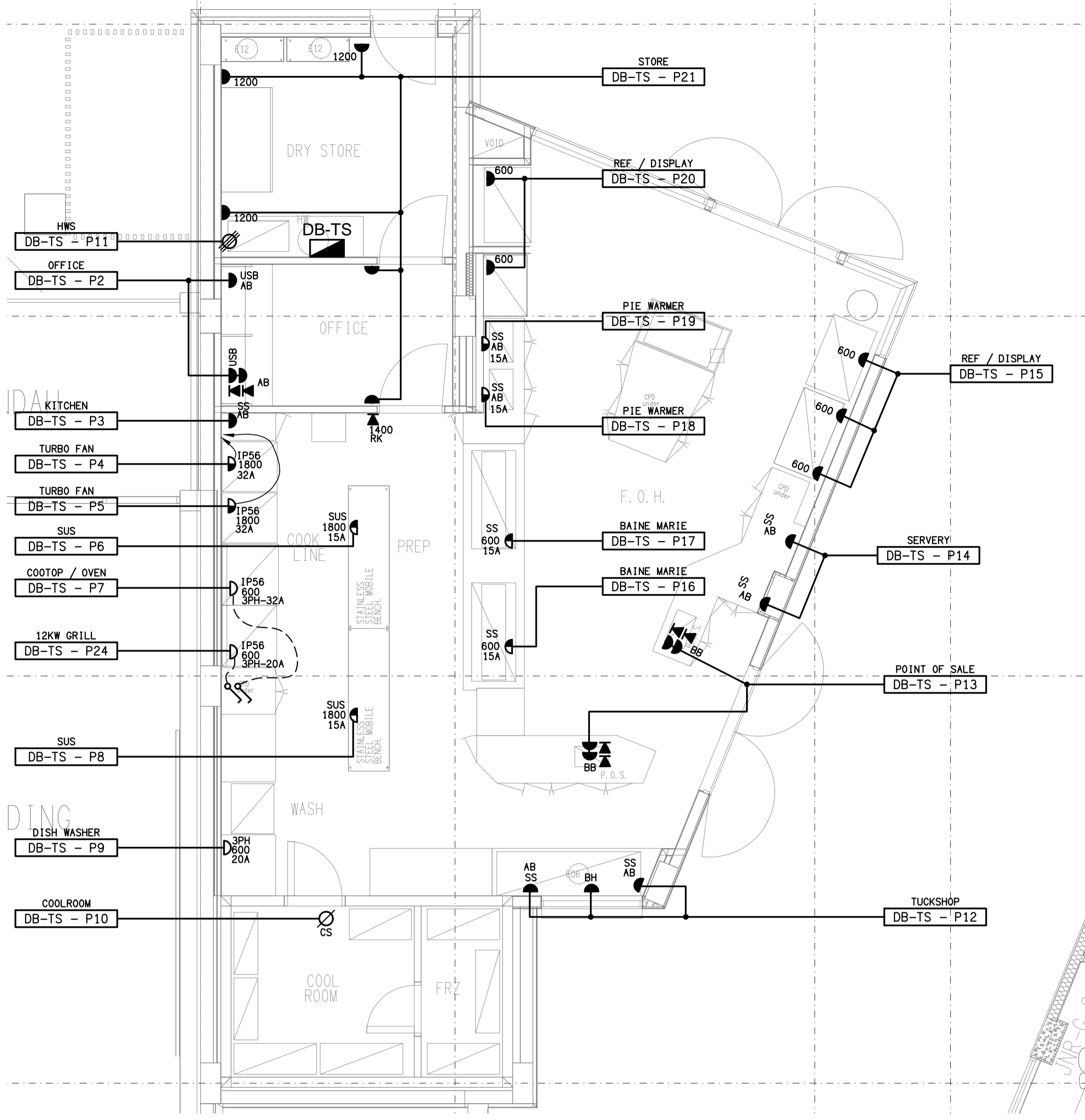
TUCKSHOP GROUND LEVEL FLOOR PLAN SCALE 1:50
